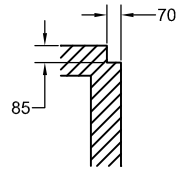
DETAIL Y Doors on Bottom Level
